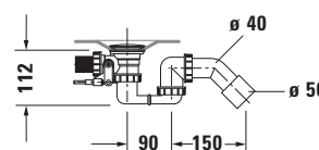
Siphon for whirltub # 760137
