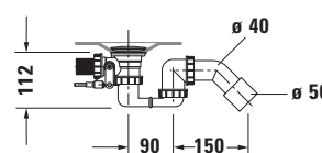
Siphon for whirltub # 760098
