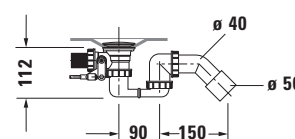
Siphon for whirltub # 760096
