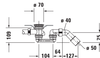
Siphon for bathtub # 700099
