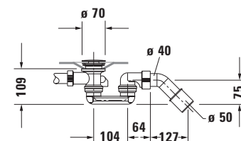
Siphon for bathtub # 700101
