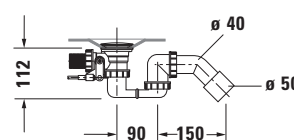
Siphon for whirltub # 760138
