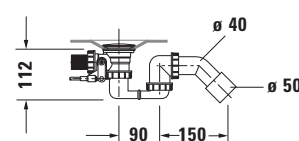
Siphon for whirltub # 760101
