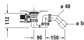
Siphon for whirltub # 760100
