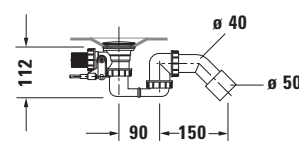
Siphon for whirltub # 760099
