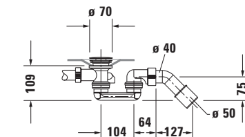
Siphon for bathtub # 700100
