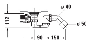
Siphon for whirltub # 760097
