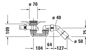
Siphon for bathtub # 700097
