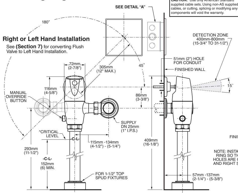
Fig. 1 Roughing-in Dimensions
