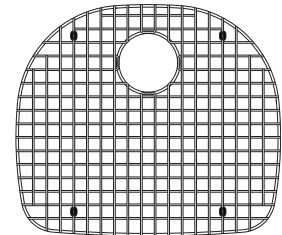
BG20S 17 1/8" x 19 9/16" x 1" 435 x 497 x 25 mm FUN#112.0055.434
