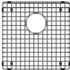
BGDS16S 15" x 15" x 1" 381 x 381 x 25 mm FUN#112.0040.600
