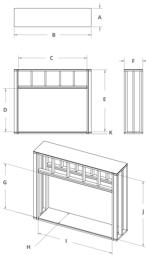
Figure 8.b Framing Box Assembly See-Through
