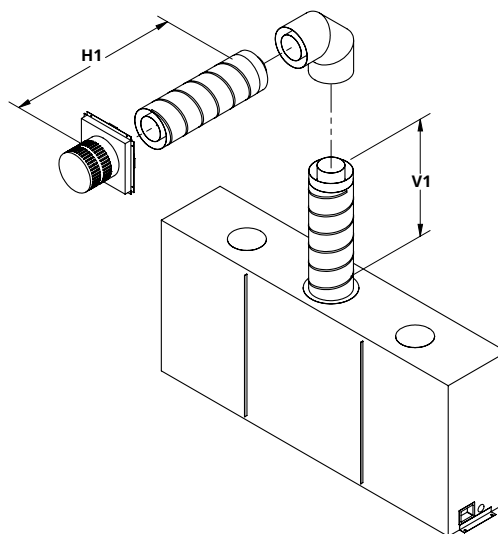
Figure 8.d Horizontal Termination - 1 Elbow
