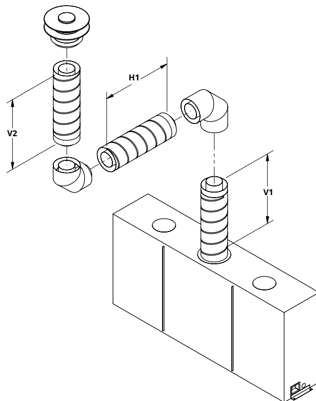
Figure 8.b Vertical Termination - 2 Elbows
