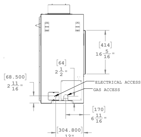
Figure 18. Gas Inlet Supply location (Single Sided)
