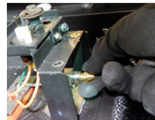
Figure 13.c Removing the orifice
