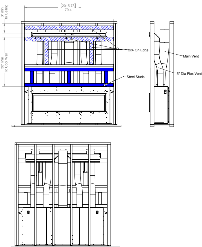
Figure 8.b.b Framing with Cool Wall Advantage
