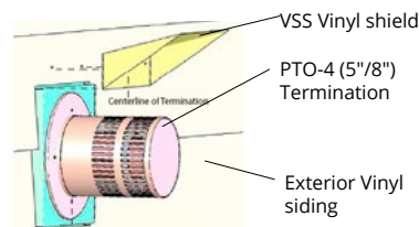
Figure 10.e Installing the VSS Vinyl Shield.
