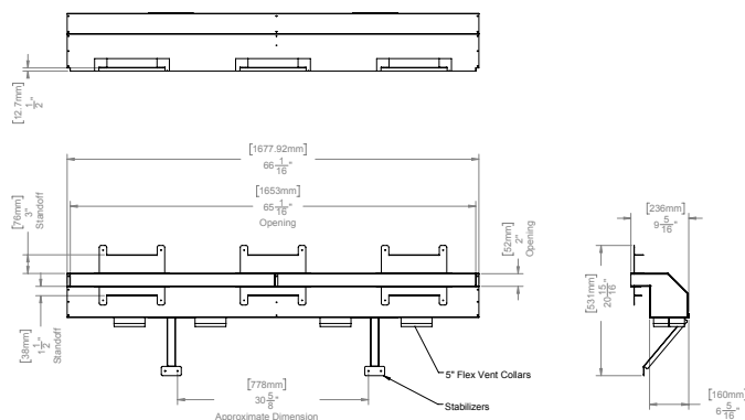
Figure 8.b.c Cool Wall Advantage vent dimensions
