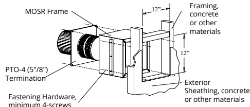
Figure 10.d Installing a PTO termination with MOSR frame.
