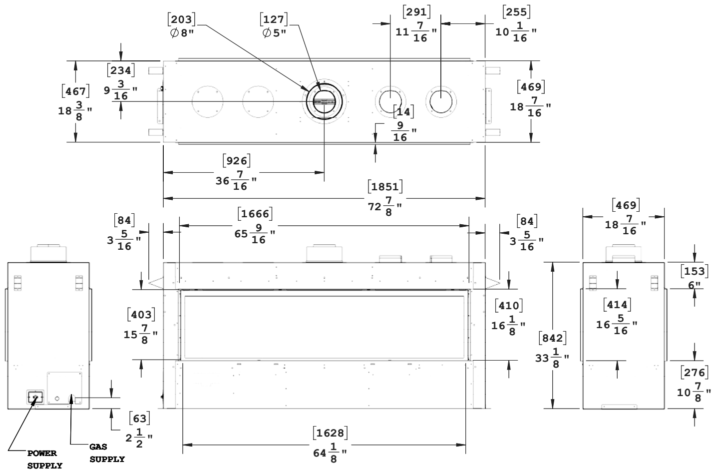
Figure 2.b DL6315ST, D6315ST Fireplace dimensions (Tolerance \pm \frac{1}{8} ").
