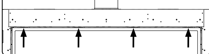
Figure 21.b Locate door buckles
