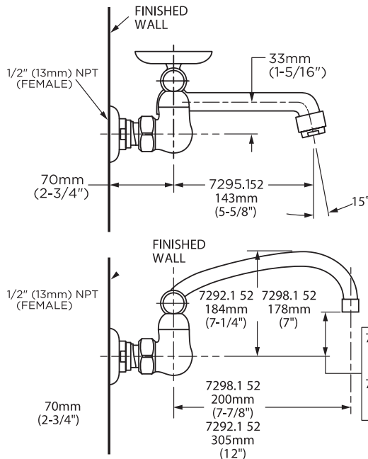
7295 152 Two-Handle Wall-Mount Sink Faucet
