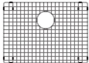
BGZ23S 16" x 21 7/8" x 1" 406 x 556 x 25 mm FUN#112.0194.731
