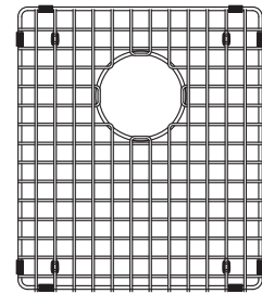
BGZ14S 14 7/8" x 12 3/4" x 1" 378 x 324 x 25 mm FUN#112.0194.703
