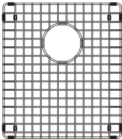
BGZ15S 16" x 13 7/8" x 1" 406 x 352 x 25 mm FUN#112.0194.710
