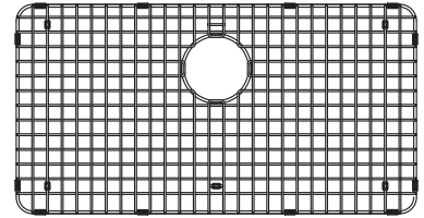
BG230S 14 1/4" x 27 1/4" x 1" 362 x 692 x 25 mm FUN# 112.0204.314
