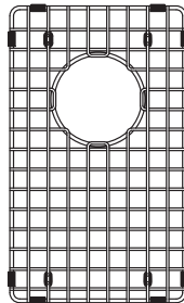
BGZ10S 14 7/8" x 8 7/8" x 1" 378 x 225 x 25 mm FUN#112.0194.732
