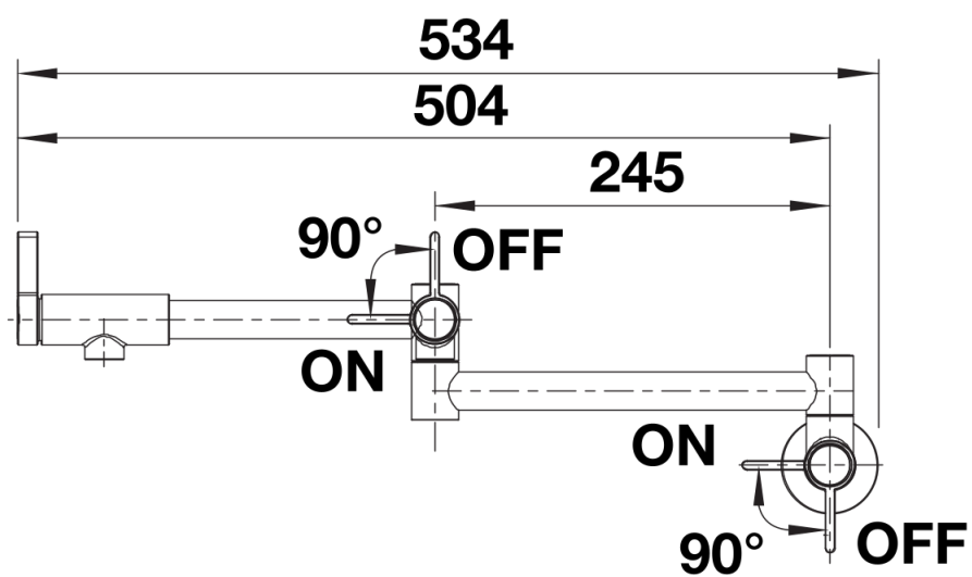
Side view hand gear 2D
