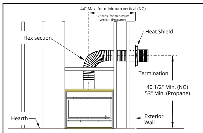
Figure 10.c Top Vented, wall mounted Multi-elbow installation. See Venting Graph for Top vent, wall mounted terminations, Figure 10 or 10b.
