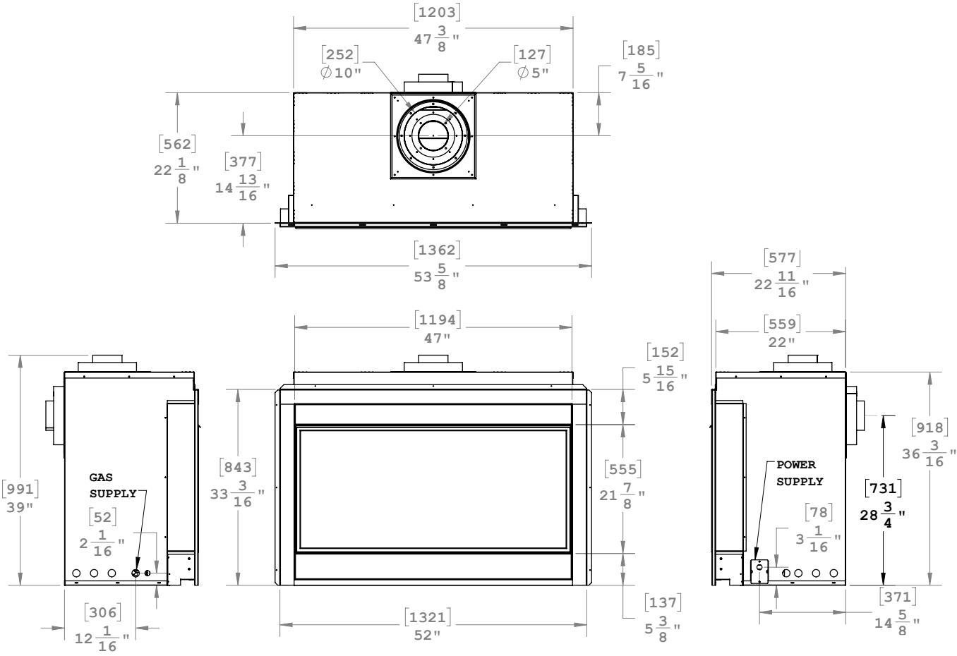
Figure 2. Fireplace dimensions (Tolerance \pm \frac{1}{16} ").
