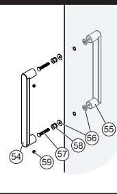
Poignée PLUS/PLUS Handle 103450-XXX *
