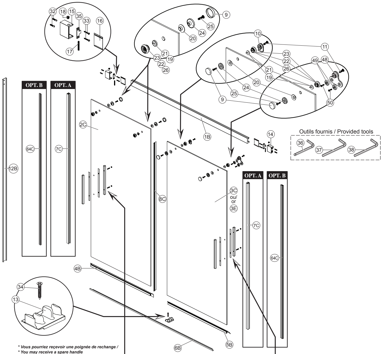
Poignée PLUS/PLUS Handle 103450-XXX *
