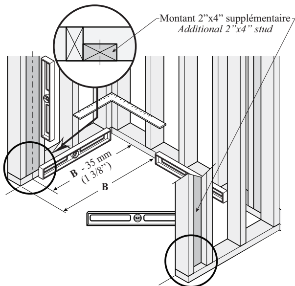
Exemple de structure de bois suggéré Wood structure suggested
