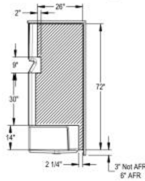
REINFORCEMENT OPTION Left Wall Shown, Symmetrical for Right
