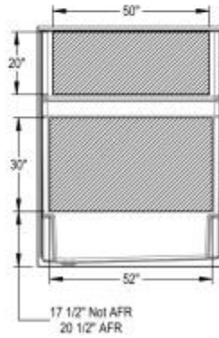
REINFORCEMENT OPTION Back Wall Shown
