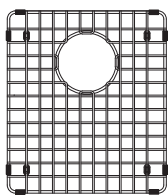
BG180S 13 5/8" x 11 7/8" x 1" 346 x 302 x 25 mm FUN#112.0055.046
