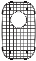
BG45S 15 7/8" x 9 9/16" x 1" 403 x 243 x 25 mm FUN#112.0036.816
