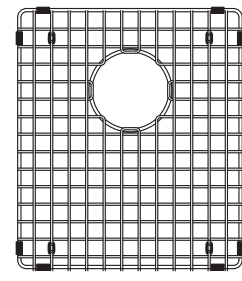
BGZ14S 14 7/8" x 12 3/4" x 1" 378 x 324 x 25 mm FUN#112.0194.703
