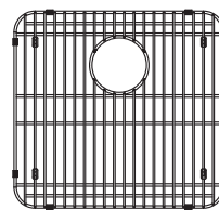
BGA1817S 15" x 16" x 1" 381 x 406 x 25 mm FUN# 112.0174.876
