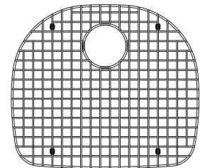
BG20S 17 1/8" x 19 9/16" x 1" 435 x 497 x 25 mm FUN#112.0055.434
