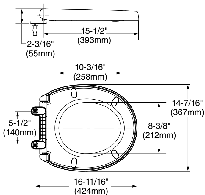
5025B65G Round Front toilet seat
